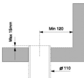
An existing outlet can be used as long as the required measurements are correct.
