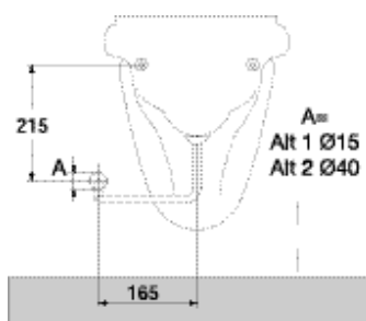
Principles for mounting the double-flush toilet
