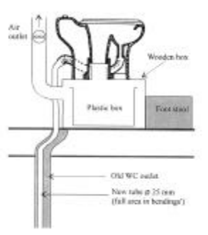
Installation with no storage space under the floor
