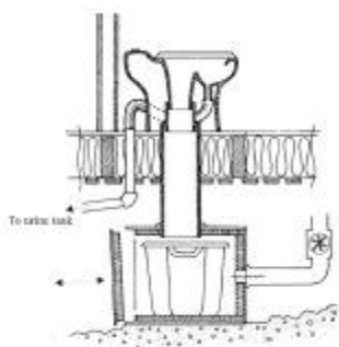
Installation with storage space under the floor
